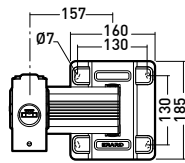
Platine murale
