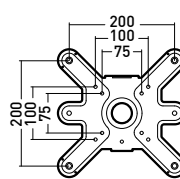
Platine murale
