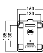
Platine murale
