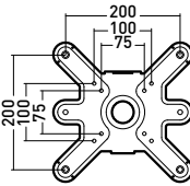
Platine murale
