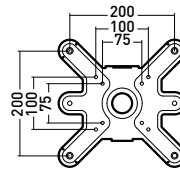
Platine murale
