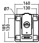
Platine murale
