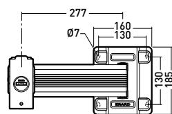
Platine murale
