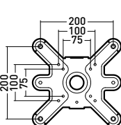
Platine murale
